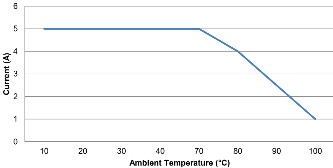
DSE9255 Temperature Derate Curve
