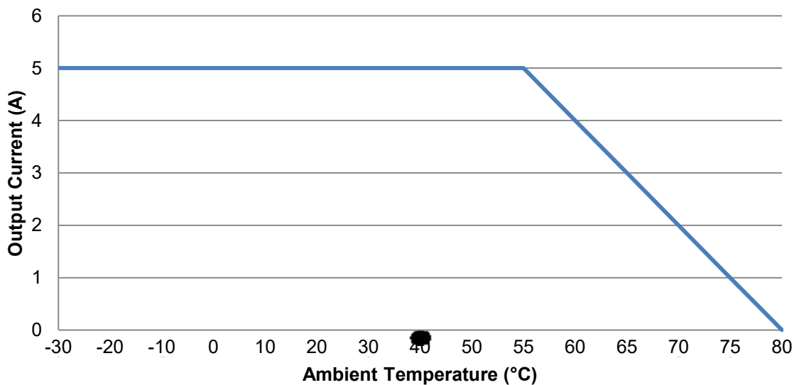
DSE9472 (MKII) Temperature Derate Curve 90 V < Vin < 305 V
